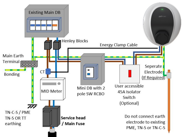
Fig. 6 Typical Solo installation layout.
