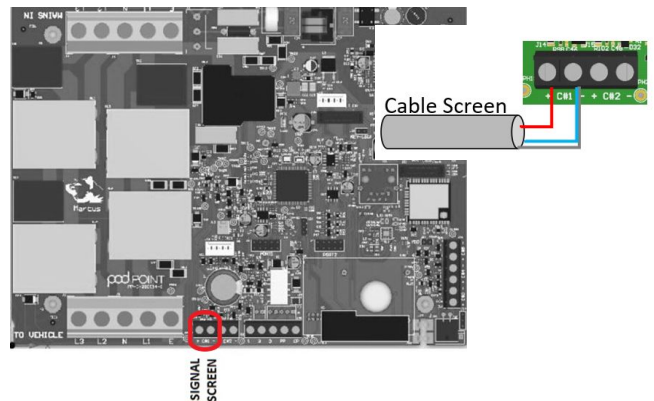
FIG.6 Energy Clamp Connection points to PCBA at J14 C#1 (Double Connector Arrangement)
