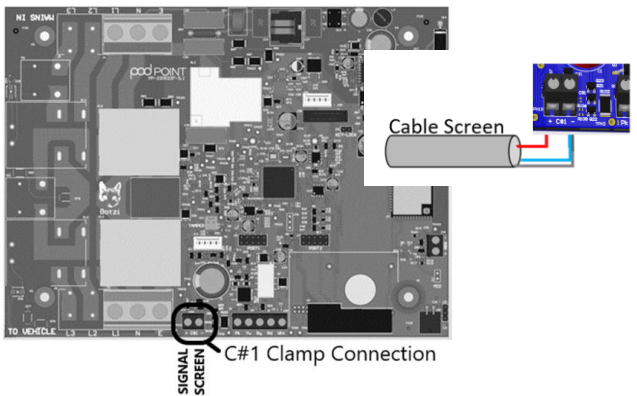
FIG.7 Energy Clamp Connection points to PCBA at J14 C#1 (Single Connector Arrangement)
