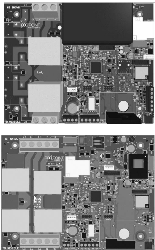
Fig 5. PCBA Variant Examples
