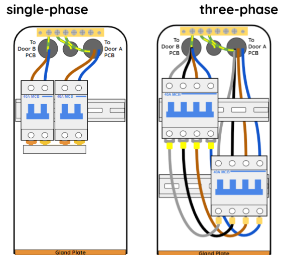
Fig 3. Initial Configuration of DBOX
