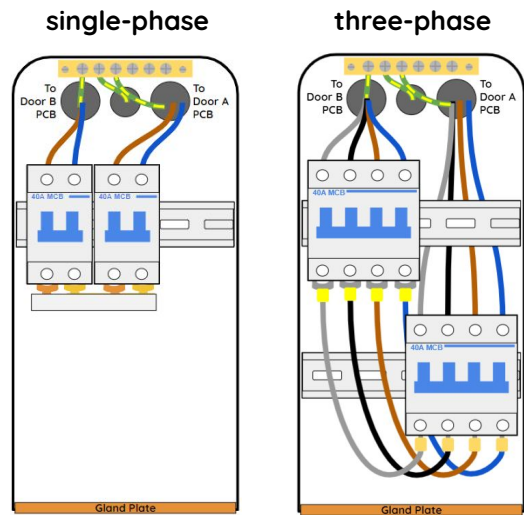
Fig 3. Initial Configuration of DBOX
