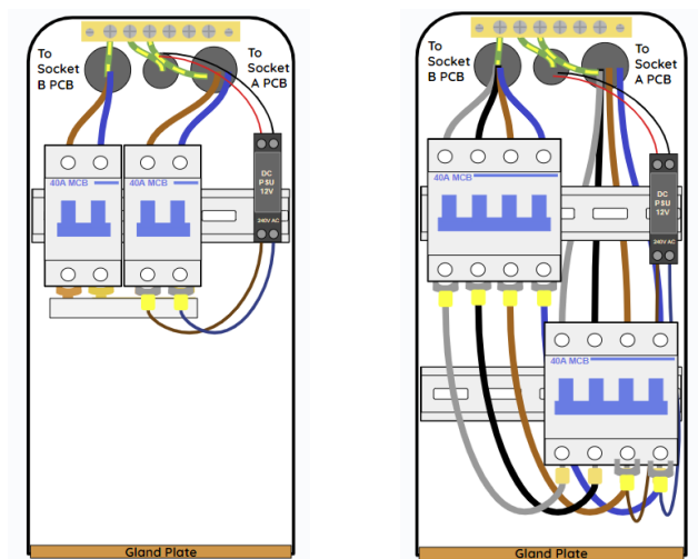
Fig 4. Initial Config of DBOX (with 12V) single-phase three-phase
